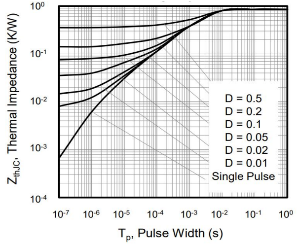
Figure 8. Transient Thermal Impedance (TO-220)
