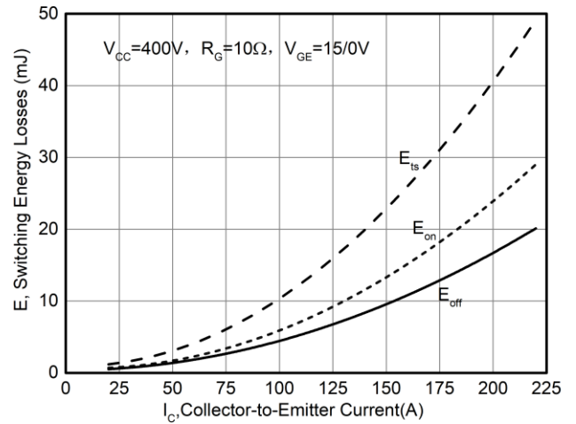
Figure 12. E_{on} , E_{off} as a function of IC ( T_j=150^\circ C )
