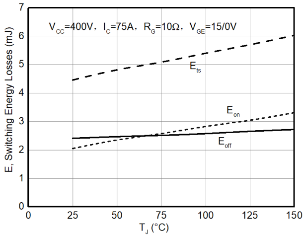
Figure 15. E_{on}, E_{off} as a function of T_j
