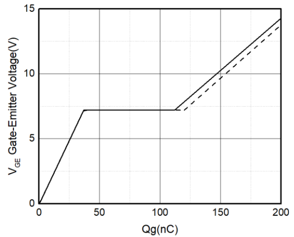
Figure 6. Typical gate charge ( I_C = 50\text{A} )
