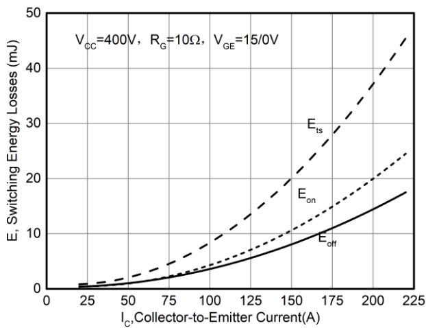
Figure 11. E_{on} , E_{off} as a function of IC ( T_j=25^\circ C )
