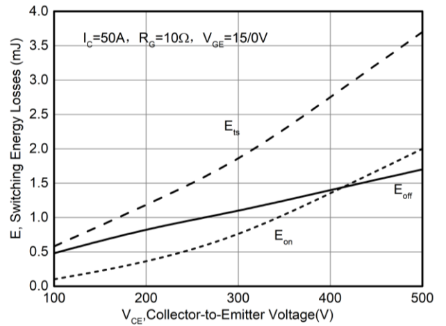
Figure 14. E_{on} , E_{off} as a function of V_{CE} ( T_j=150^\circ\text{C} )
