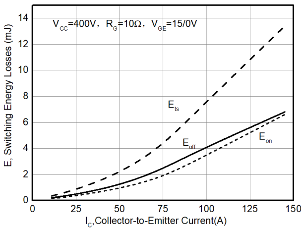
Figure 11. E_{on} , E_{off} as a function of I_C ( T_j=25^\circ C )
