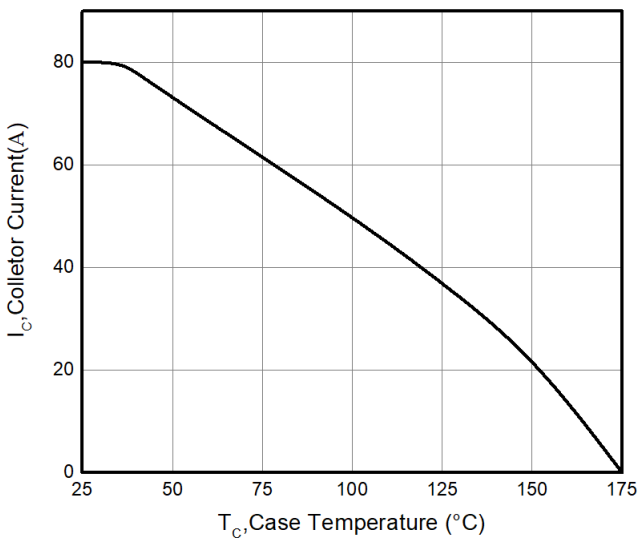
Figure 17. Collector current as a function of case temperature ( V_{GE} \geq 15\text{V} , T_j \leq 175^\circ\text{C} )
